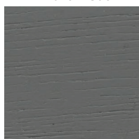
Andromeda
